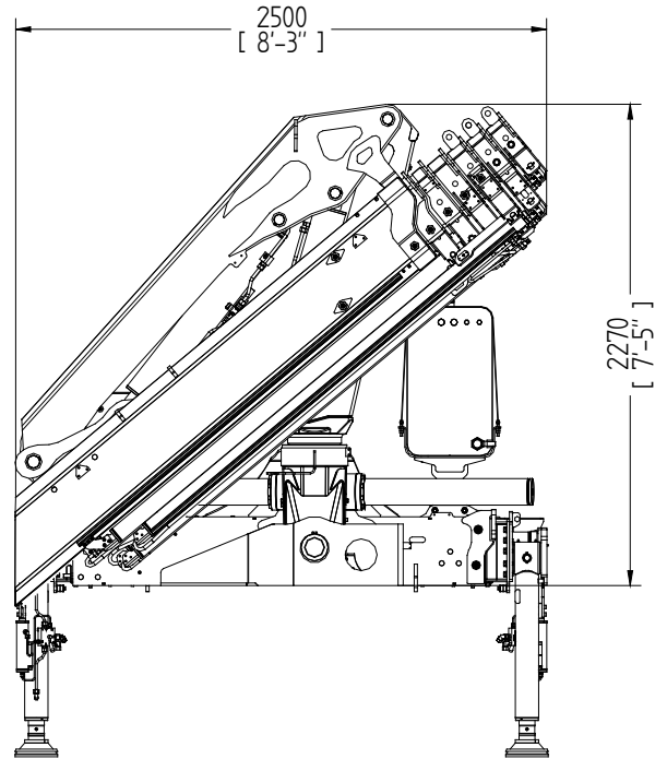
rear truck
